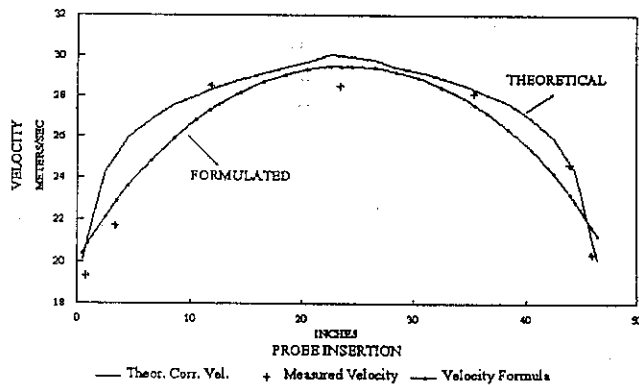
FIGURE 4 VELOCITY PROFILE
