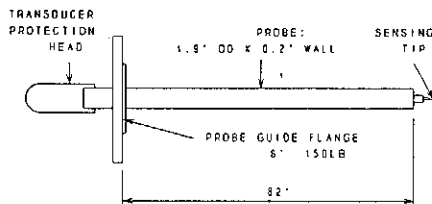
FIGURE 3 Probe Details
