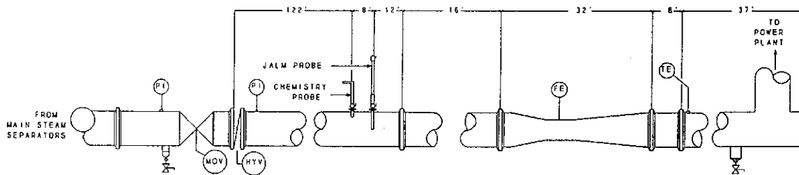
FIGURE 2 Location of JALM Probe
