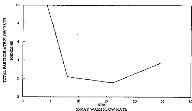
FIGURE 6 Effects of Spray Wash on Particulate
