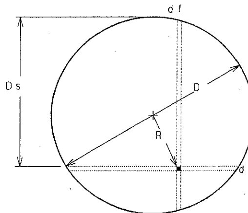
FIGURE 5 Differential Area of pipe's cross section
