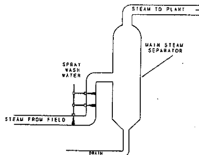
FIGURE 1 Spray Wash & Separator
